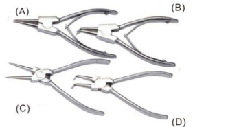
4件套挡圈钳 4PC Circclip Pliers
